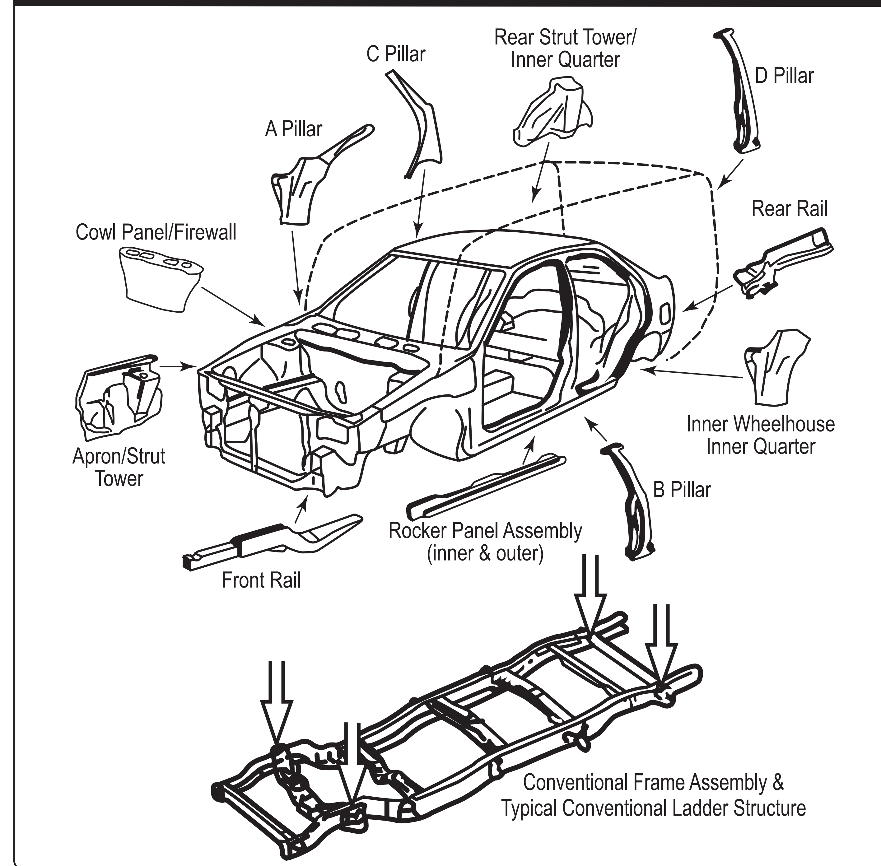
TYPICAL UNIBODY ON CONVENTIONAL FRAME STRUCTURE
